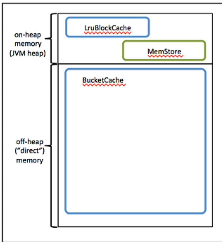
Figure 1: Relationship among Different BlockCache Implementations and MemStore
