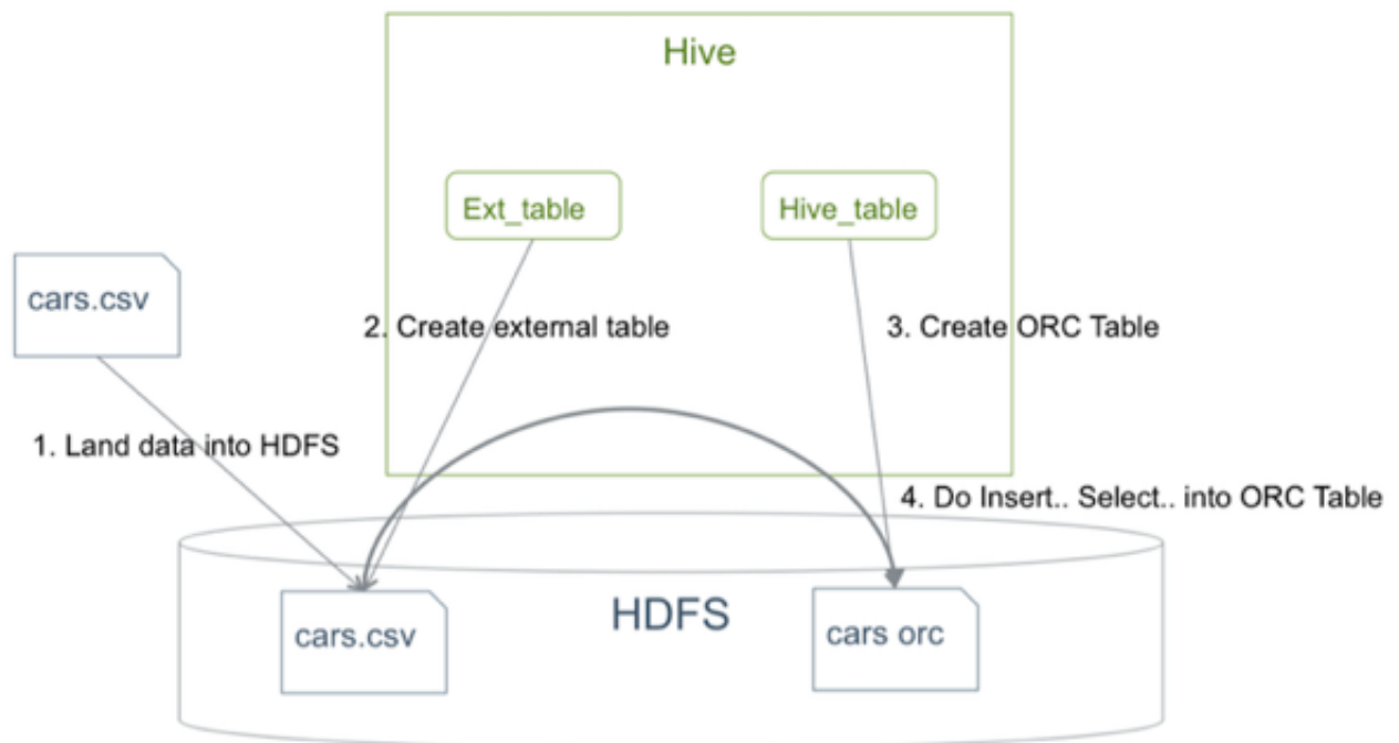
Figure 2.1. Example: Moving .CSV Data into Hive
