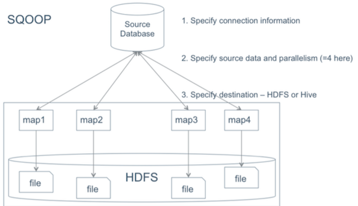
Figure 2.2. Using Sqoop to Move Data into Hive
