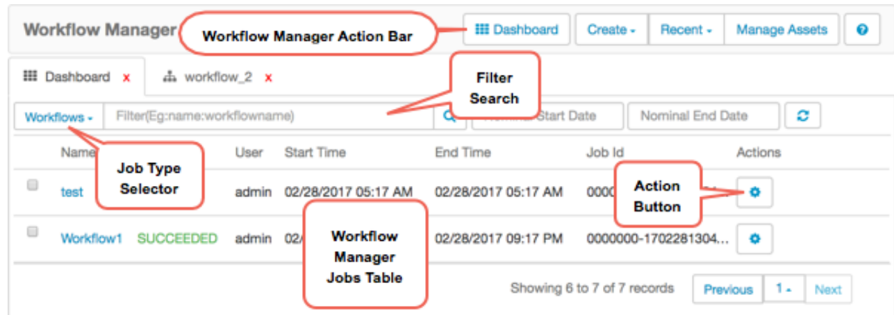
Figure 3.2. Workflow Manager Dashboard Component
