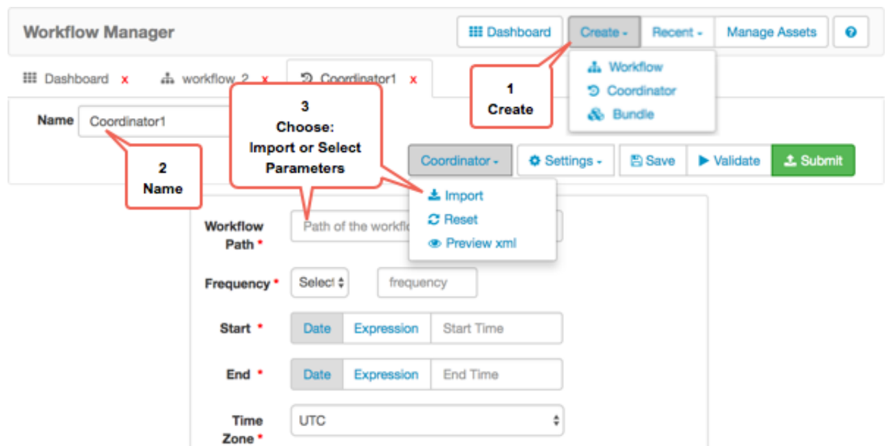
Figure 4.10. Creating a Coordinator
