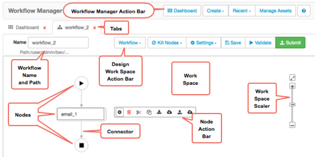
Figure 3.1. Workflow Manager Design Component
