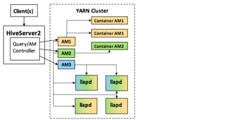
Figure 2.10. LLAP on Your Cluster
