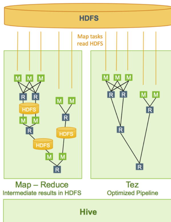
Figure 3.1. Tez Query Execution Compared to MapReduce
