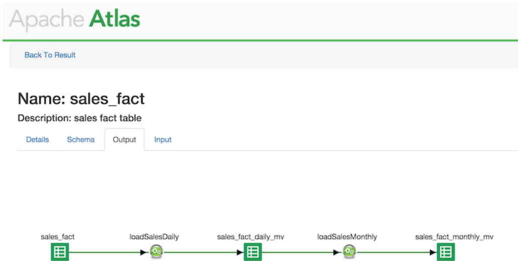
Figure 3.6. Output Tab
