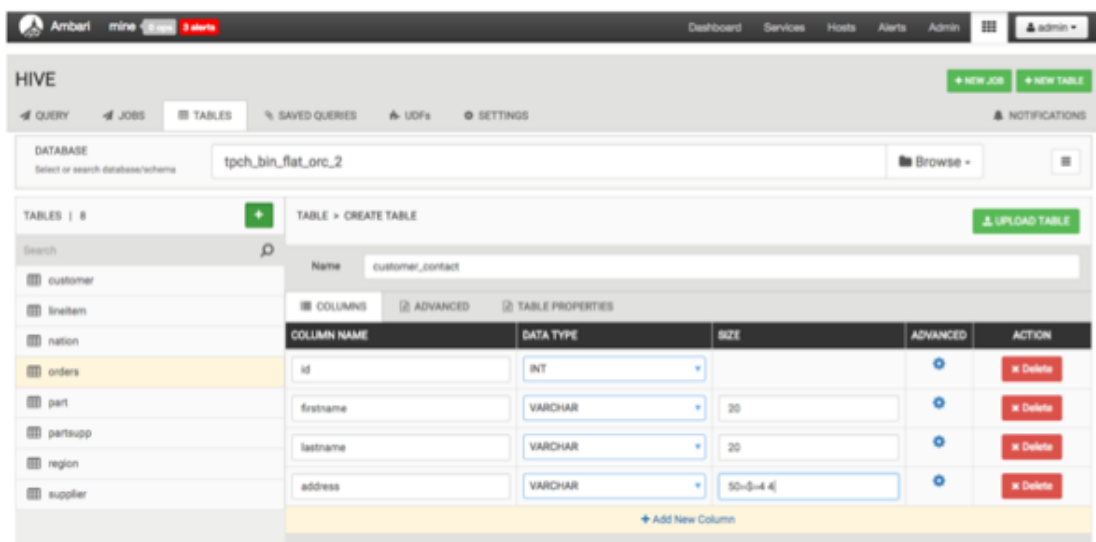
Figure 6.13. Example of Creating a Table Form
